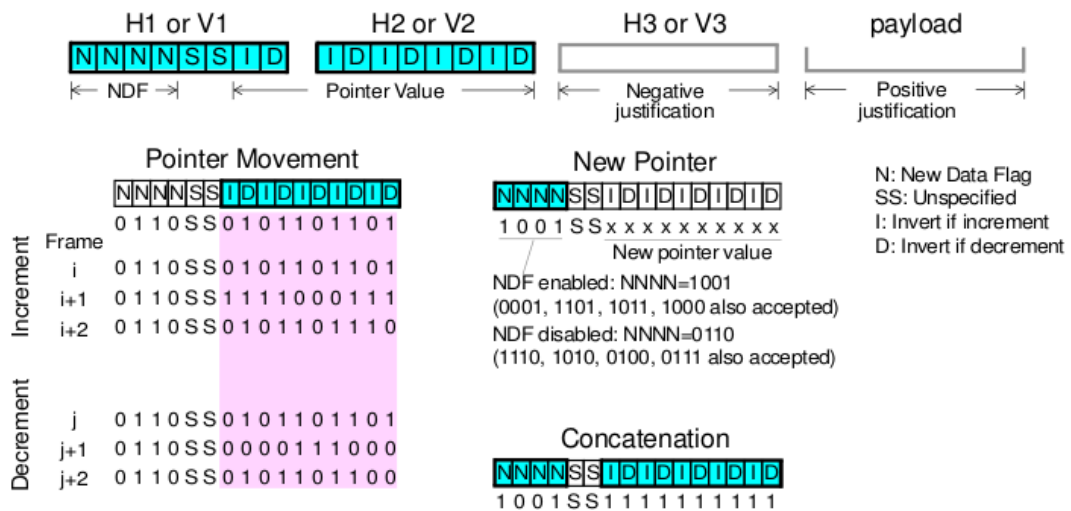
Figure 4 Pointer formats, codification and procedures.
